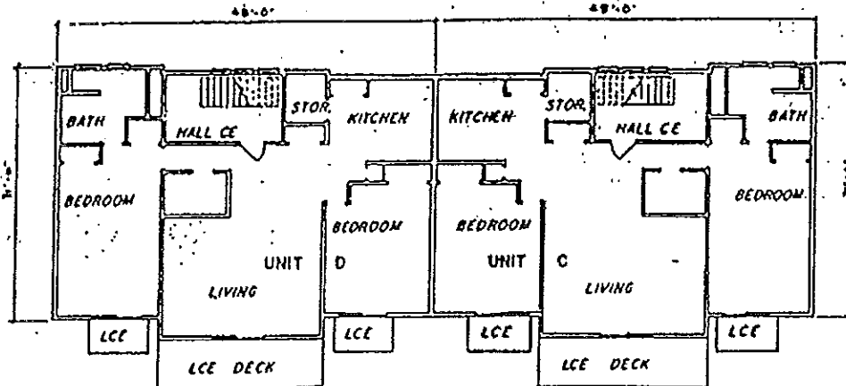
SECOND FLOOR PLAN FOR BLDGS. 10, 11, & 12
