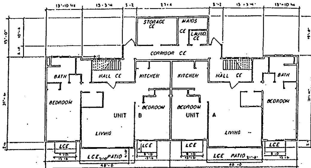
FIRST FLOOR PLAN FOR BLDGS. 10, 11, & 12
